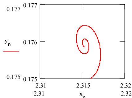
Fig. 5 The damped oscillation path ([X], [Y])
