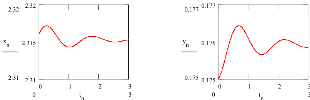
Fig. 4 The damped oscillations in chemical reactions: the concentration of the intermediaries X, and the concentration of the intermediaries Y
