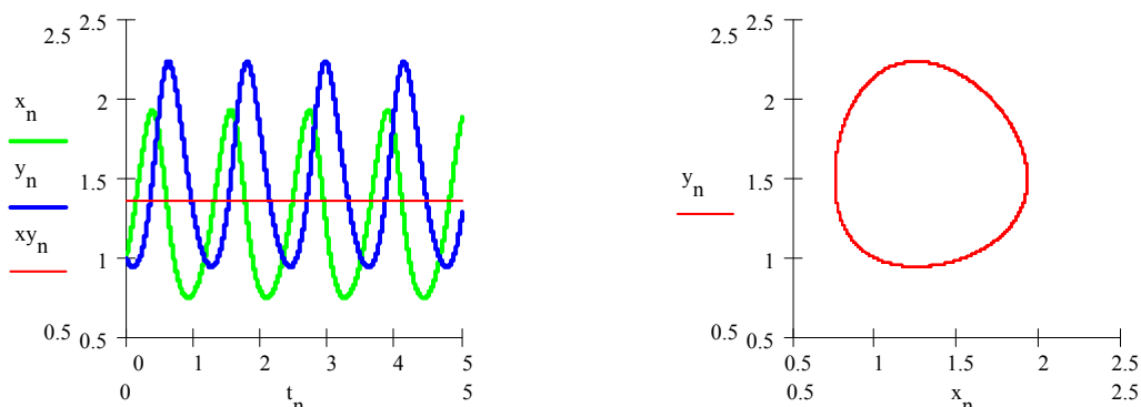
Fig. 2 The oscillation of the intermediaries and the variation path ([X],[Y]) in L-V mechanism
