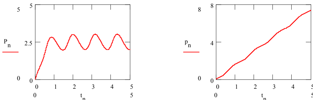
Fig. 3 The variation of the product concentration and storage in L-V mechanism
