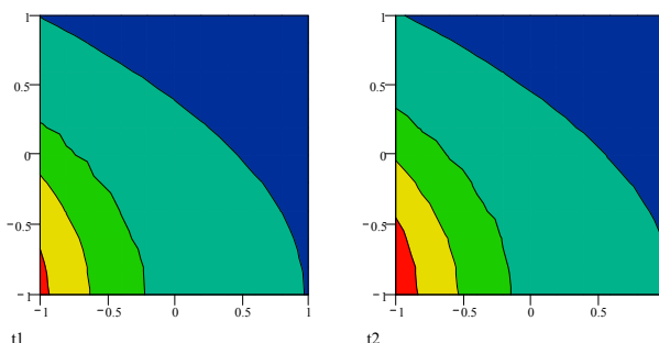
Fig. 1 Concentration gradient in an oscillating reaction at the t , and at the t + \Delta t moments; Avi animation: http://lori.east.utcluj.ro/free/RO.avi
