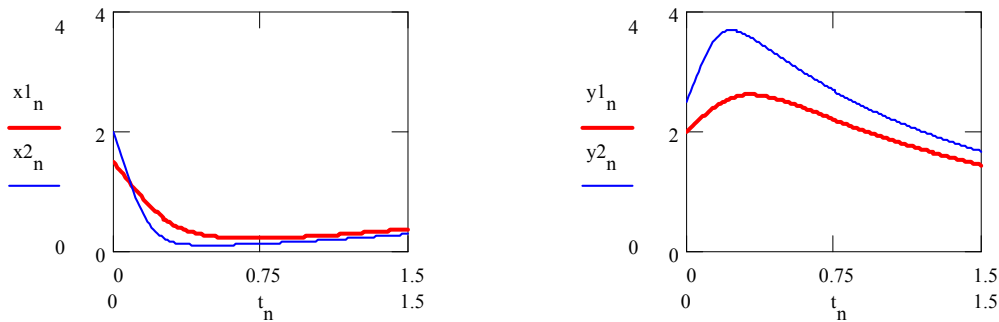
Fig. 7 The concentrations of the intermediaries up to the attractor for two cases with different initial conditions
