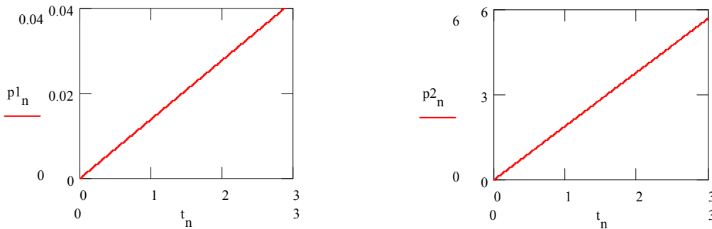
Fig. 6 The linear variation of the amount of products in damped oscillating reactions
