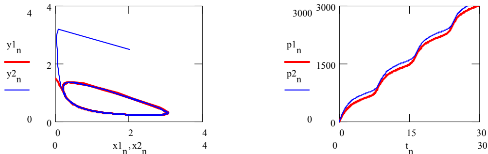
Fig. 10 Convergence at attractor of brusselator system independent from initial conditions and different quantities of resulted product
