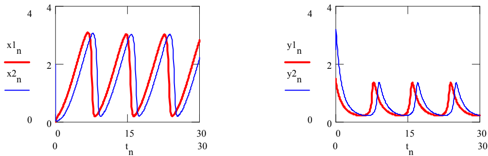
Fig. 9 The periodical evolution having the same oscillation period T = 0.226 of [X] and [Y] , for two cases having different initial conditions
