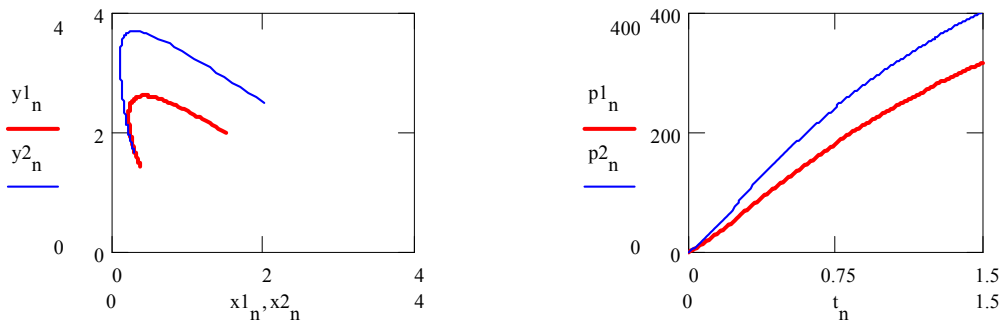
Fig. 8 The entrance of [Y] related to [X] on the same gravitational orbit for different product quantities obtained in two cases having different initial conditions
